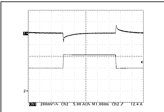
Figure 15: Output voltage response to step-change in load current (50%-75%-50% of Iout(max); di/dt = 0.1A/\mu s ). Load cap: 10 \mu F, 100 m \Omega ESR tantalum capacitor and 1 \mu F ceramic capacitor. Ch 1: Vout (200mV/div), Ch 2: Iout (5A/div).
