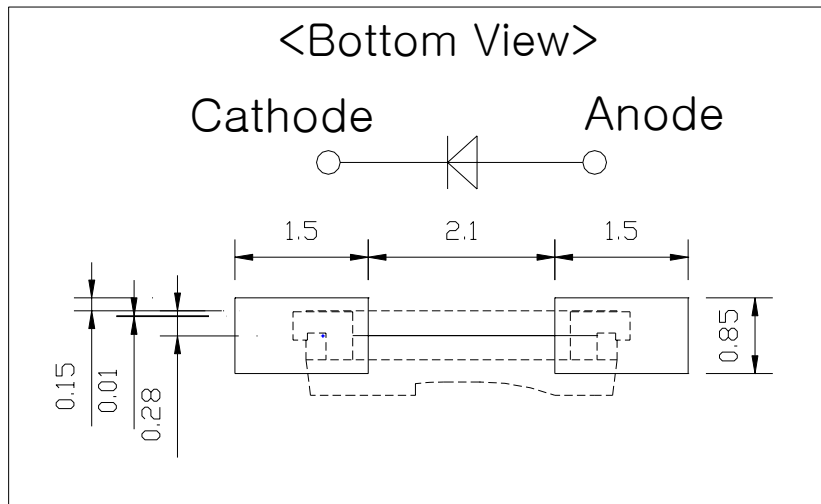
Recommended solder Pattern
