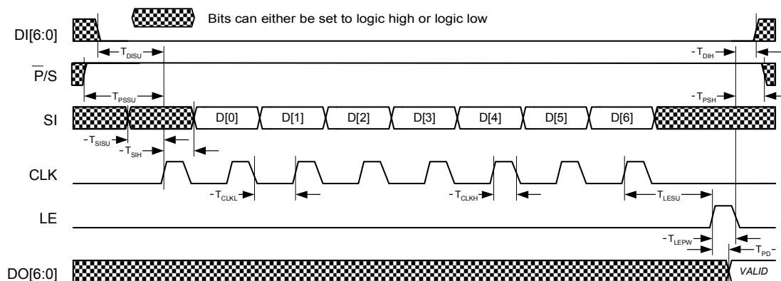
Figure 15. Serial Timing Diagram
