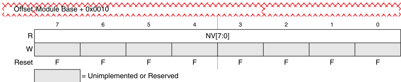
Figure 27-22. Flash Option Register (FOPT)
