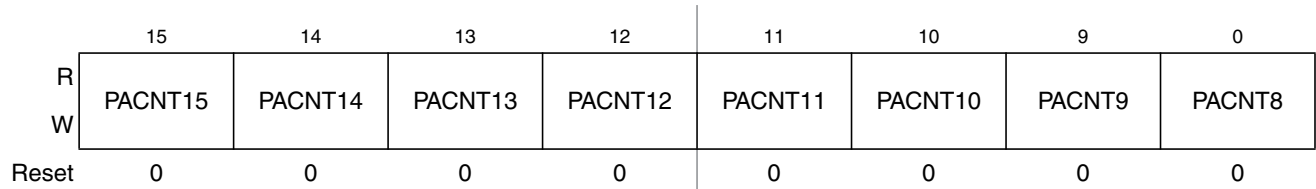
Figure 22-26. Pulse Accumulator Count Register High (PACNTH)
