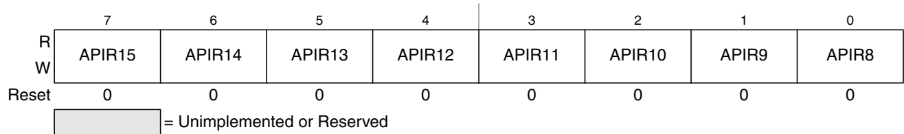
Figure 23-5. Autonomous Periodical Interrupt Rate High Register (VREGAPIRH)
