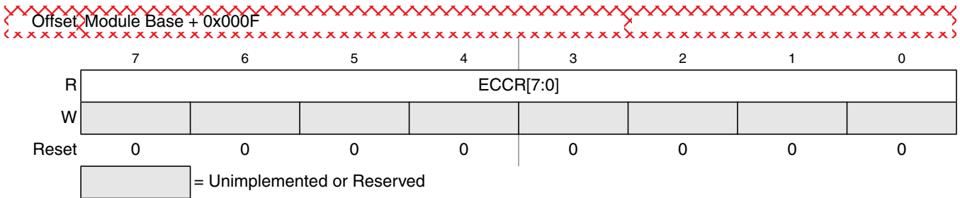
Figure 29-21. Flash ECC Error Results Low Register (FECCRLO)
