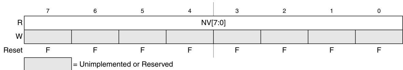
Figure 28-22. Flash Option Register (FOPT)
