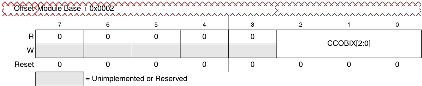
Figure 29-7. FCCOB Index Register (FCCOBIX)
