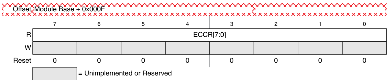
Figure 27-21. Flash ECC Error Results Low Register (FECCRLO)
