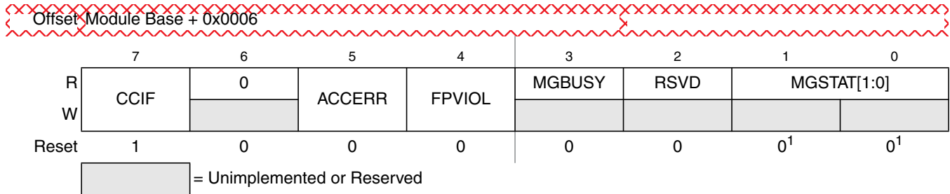
Figure 29-11. Flash Status Register (FSTAT)
