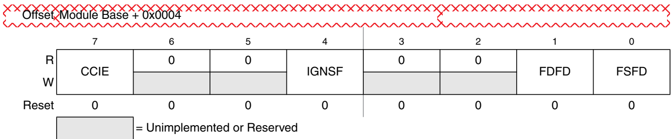
Figure 26-9. Flash Configuration Register (FCNFG)
