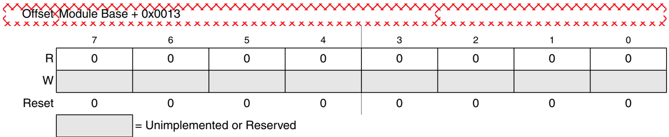
Figure 26-25. Flash Reserved 2 Register (FRSV 2 )
