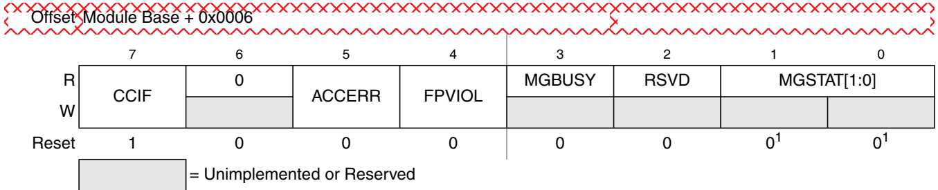
Figure 27-11. Flash Status Register (FSTAT)
