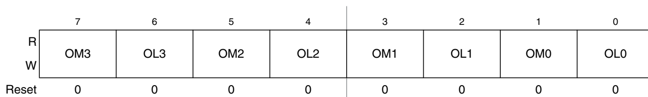
Figure 22-15. Timer Control Register 2 (TCTL2)
