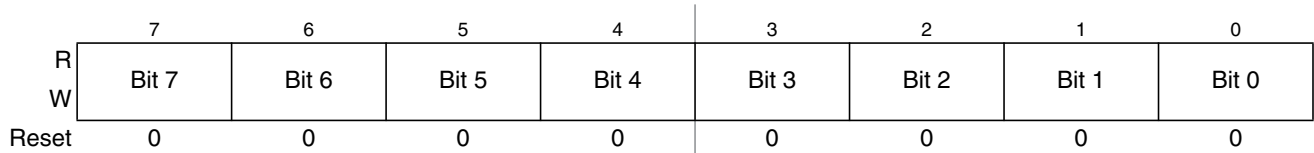
Figure 14-20. Timer Input Capture/Output Compare Register 0 Low (TC0)
