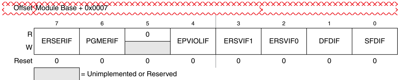
Figure 26-12. Flash Error Status Register (FERSTAT)
