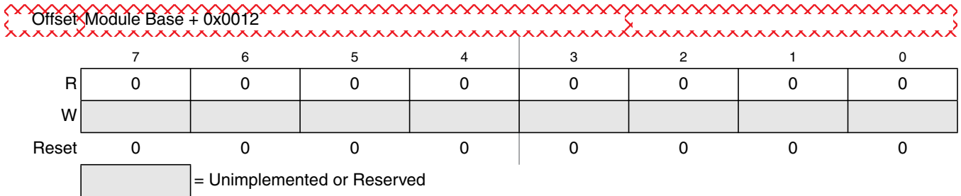
Figure 29-24. Flash Reserved 1 Register (FRSV 1 )
