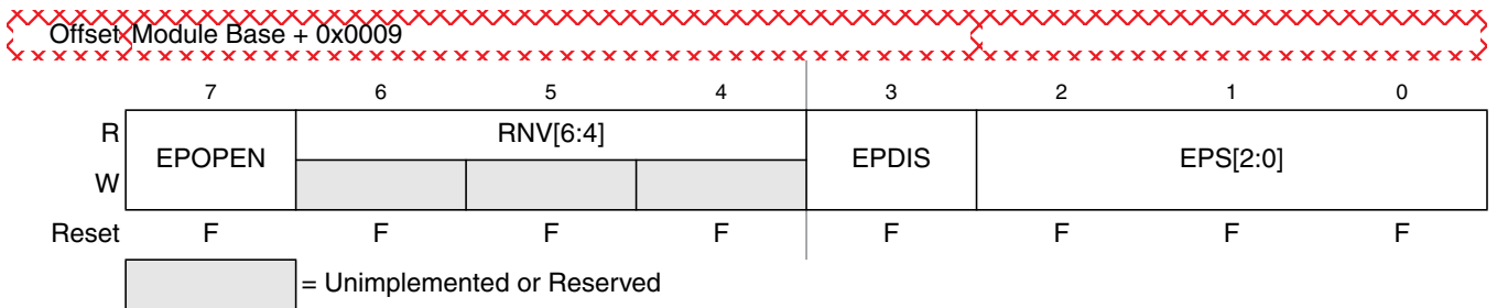
Figure 27-15. EEE Protection Register (EPROT)
