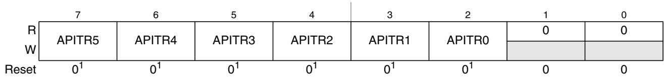
Figure 23-4. Autonomous Periodical Interrupt Trimming Register (VREGAPITR)
