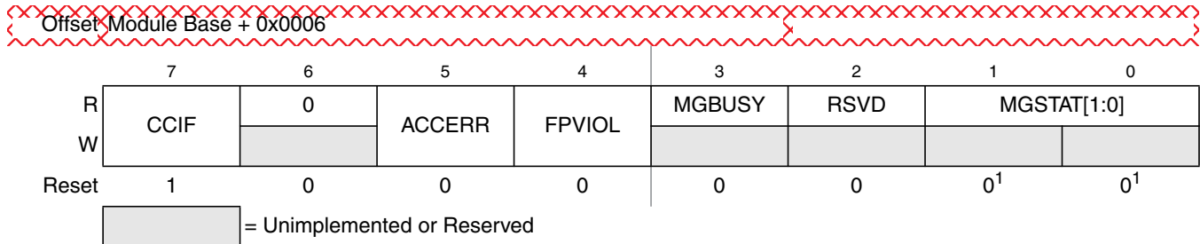
Figure 26-11. Flash Status Register (FSTAT)
