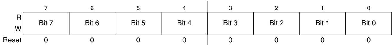
Figure 14-22. Timer Input Capture/Output Compare Register 1 Low (TC1)
