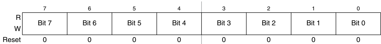
Figure 14-24. Timer Input Capture/Output Compare Register 2 Low (TC2)
