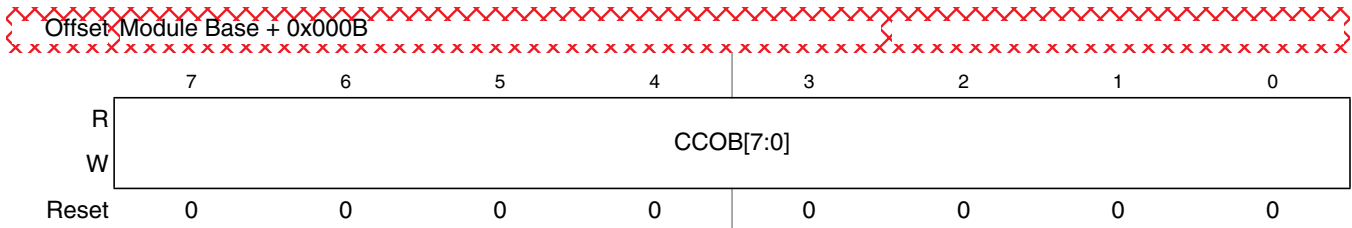
Figure 29-17. Flash Common Command Object Low Register (FCCOBLO)
