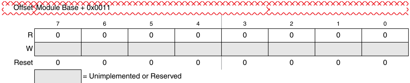
Figure 29-23. Flash Reserved 0 Register (FRSV 0 )
