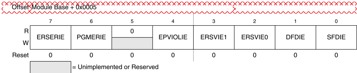
Figure 29-10. Flash Error Configuration Register (FERCNFG)
