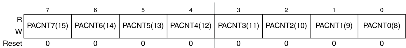
Figure 14-37. Pulse Accumulators Count Register 3 (PACN3)
