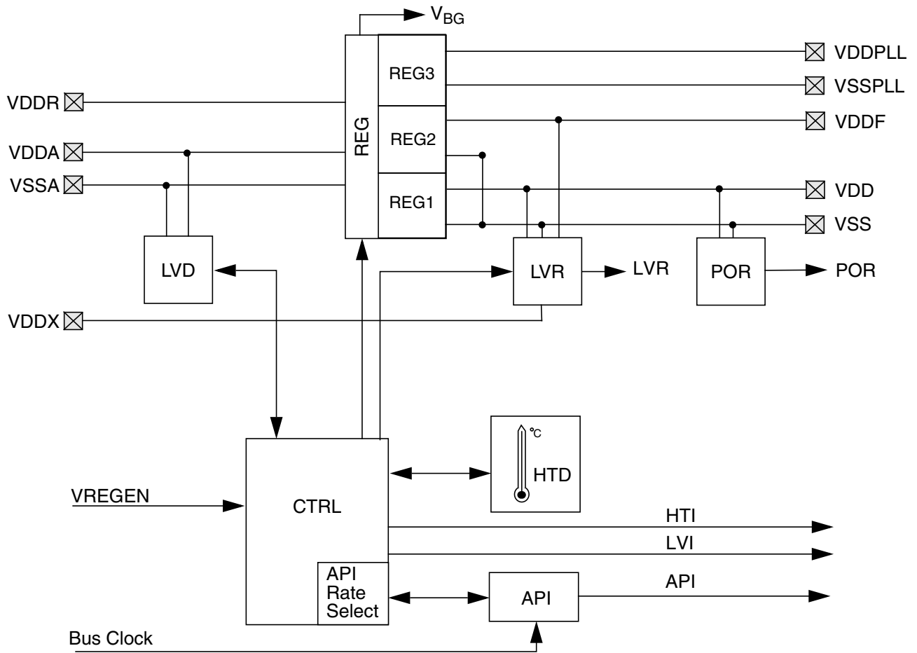
Figure 23-1. VREG_3V3 Block Diagram
