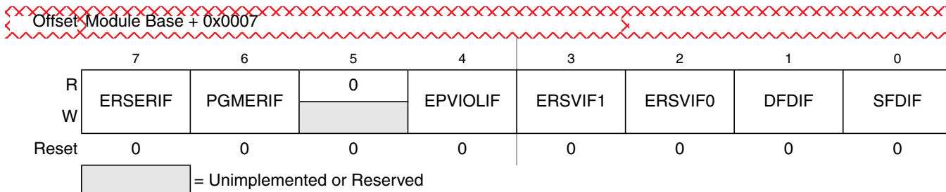
Figure 27-12. Flash Error Status Register (FERSTAT)
