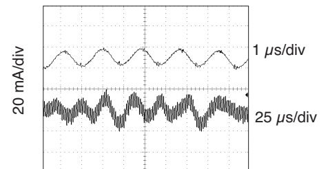
MOR2812D Input Ripple ( I_{in} ) FIGURE 49
