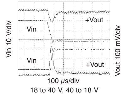
MOR2812D Step Line Response FIGURE 52
