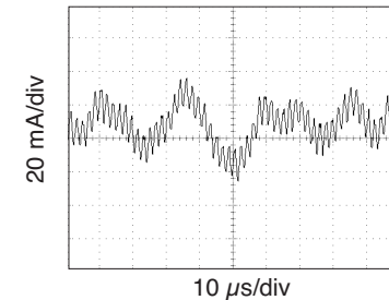
MOR2815S Input Ripple (lin) FIGURE 37
