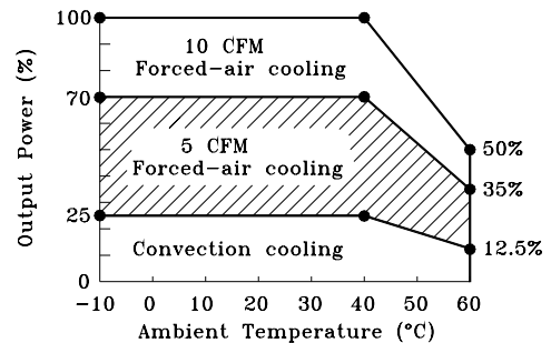
DERATING CURVE
