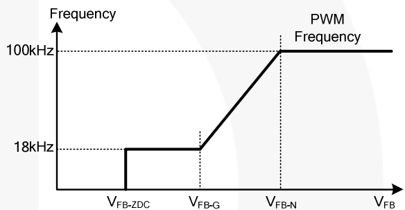
Figure 25. PWM Frequency
