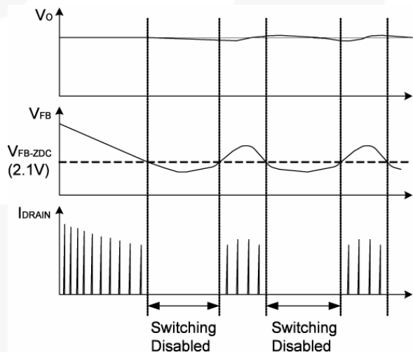
Figure 26.Burst Mode Operation
