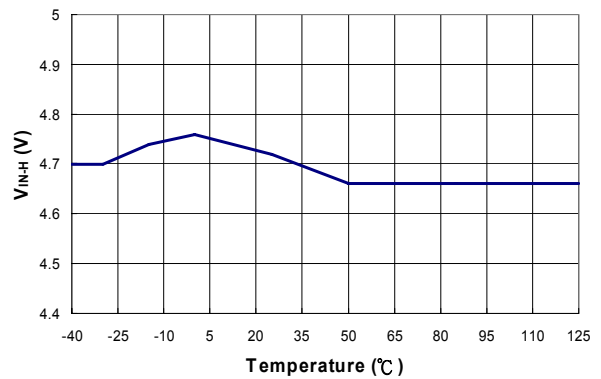
Figure 16. V_{IN-H} vs. Temperature
