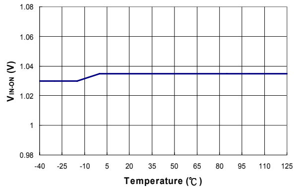
Figure 14. V_{IN-ON} vs. Temperature
