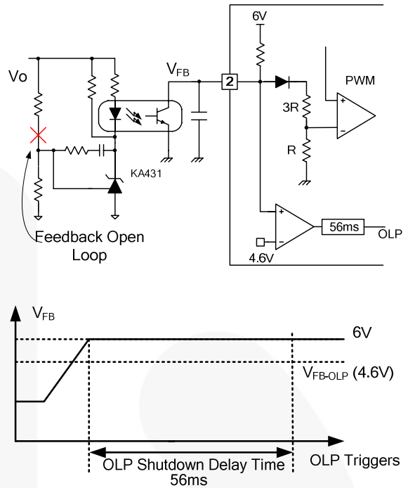
Figure 29. OLP Operation
