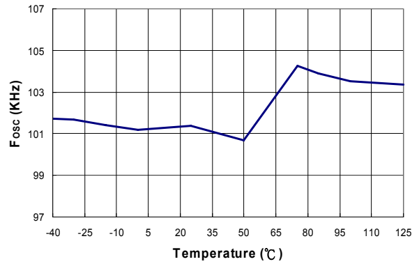
Figure 12. f_{osc} vs. Temperature
