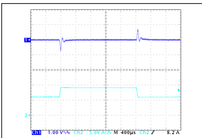
Figure 5: Output voltage response to step-change in load current (50%-75%-50% of Iout(max); dI/dt = 0.1 A/μs). Load cap: 1 μF ceramic capacitor. Ch 1: Vout (1 V/div), Ch 2: Iout (5 A/div).
