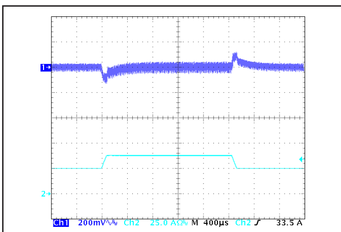
Figure 5: Output voltage response to step-change in load current (50%-75%-50% of I out (max); dI/dt = 0.1 A/μs). Load cap: 1 μF ceramic capacitor. Ch 1: Vout (200 mV/div), Ch 2: Iout (25 A/div).
