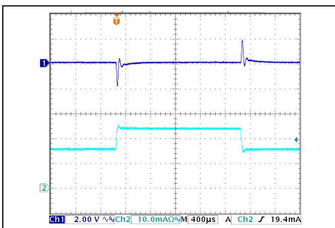
Figure 5: Output voltage response to step-change in load current (50%-75%-50% of I out (max); dI/dt = 0.1 A/μs). Load cap: 1 μF ceramic capacitor. Ch 1: Vout (2 V/div), Ch 2: Iout (10 mA/div).
