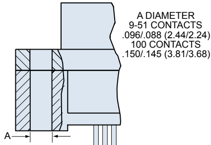
NN Style Thru-Hole, No Hardware
