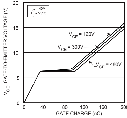
FIGURE 4, Gate charge
