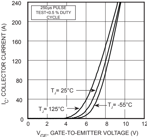
FIGURE 3, Transfer Characteristics
