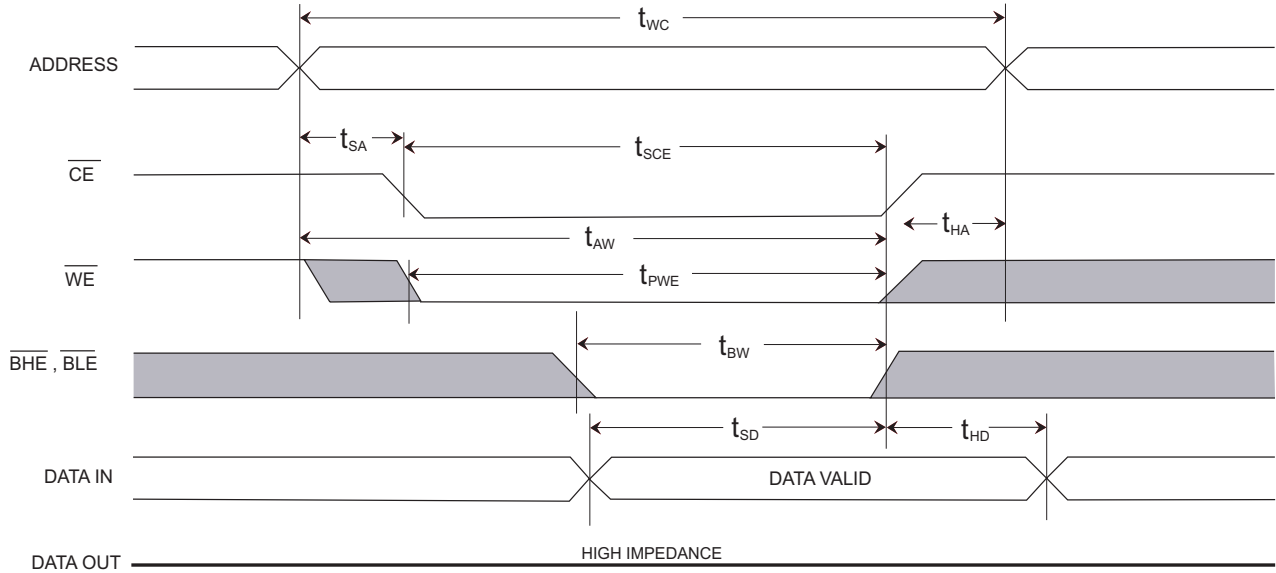
Figure 10. SRAM Write Cycle #2: \overline{\text{CE}} Controlled [18, 26, 27, 28]
