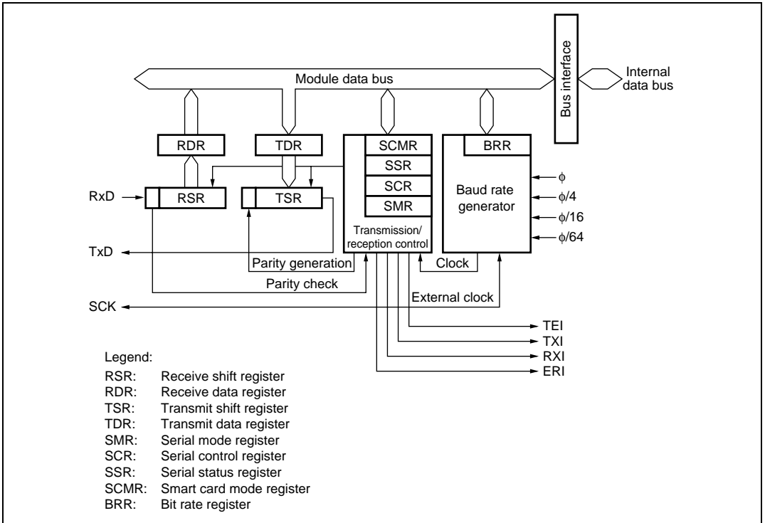
Figure 13.2 Block Diagram of SCI_1 or SCI_2
