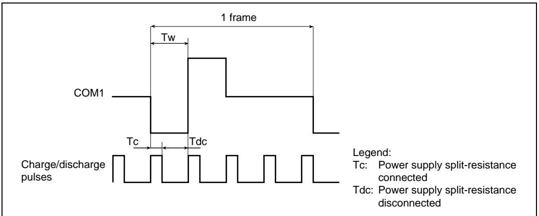
Figure 17.2 A Waveform 1/2 Duty 1/2 Bias
