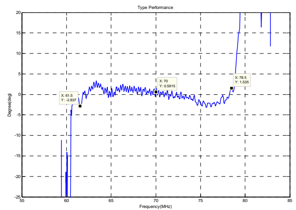
Phase Linearity(f0±8.5MHz)
