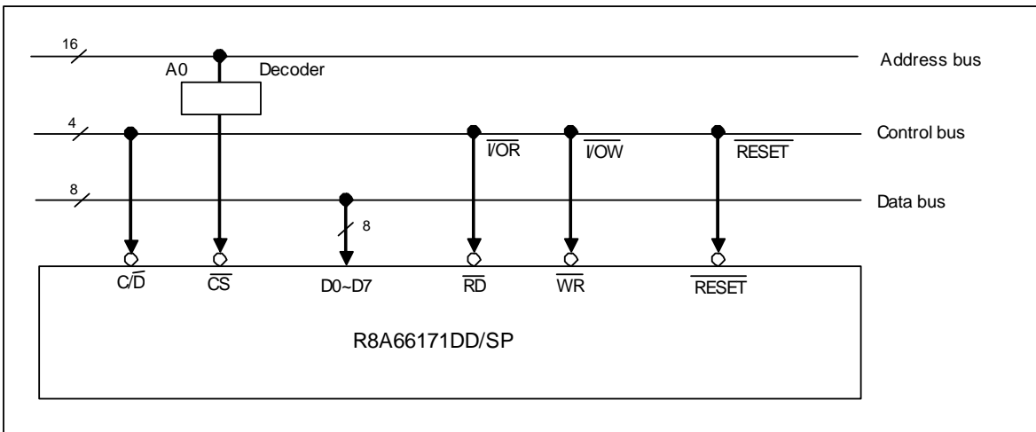
Fig.1 Interface between the R8A66171 and MCU system bus
