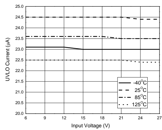
Figure 15. UVLO Current vs. Input Voltage
