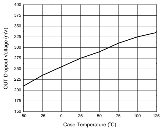
Figure 19. OUT Dropout Voltage vs. Case Temperature
