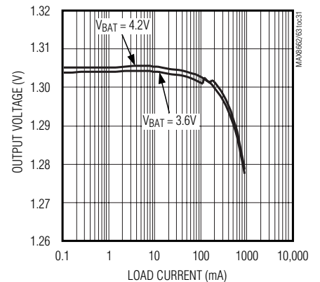
OUT2 REGULATOR LOAD REGULATION
