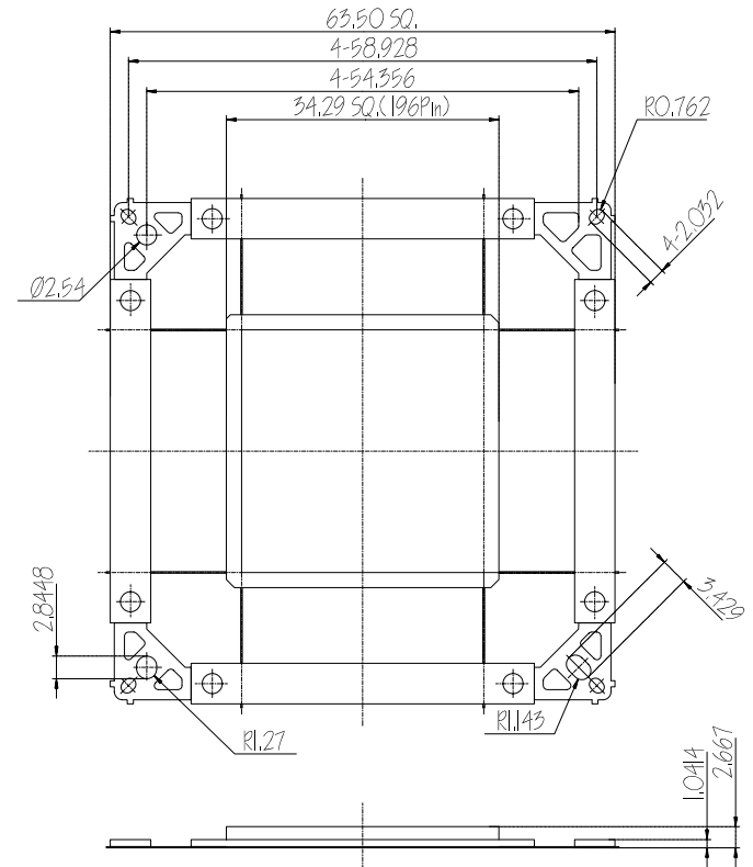
MATCHING IC PKG (Reference)
