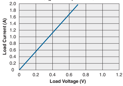
Typical Load Current vs. Load Voltage ( T_A=25°C, I_F=10mA )
