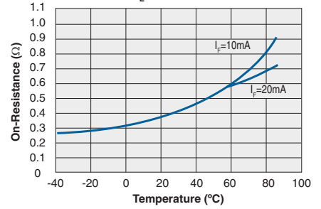
Typical On-Resistance vs. Temperature ( I_L=Max\ Rated )
