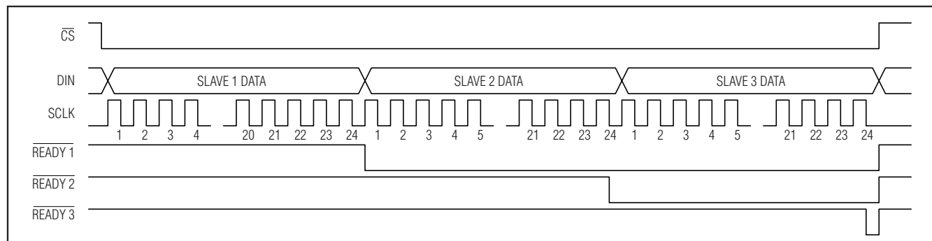
Figure 4. \overline{READY} Timing
