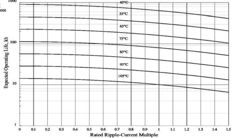
Type 381EL Operating Life in Kilohours vs Ripple Current
