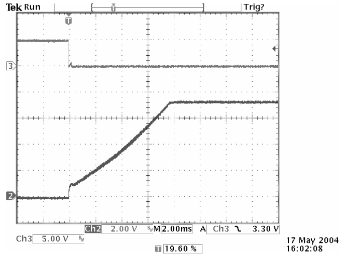
Turn-on from Enable (Vin present)
