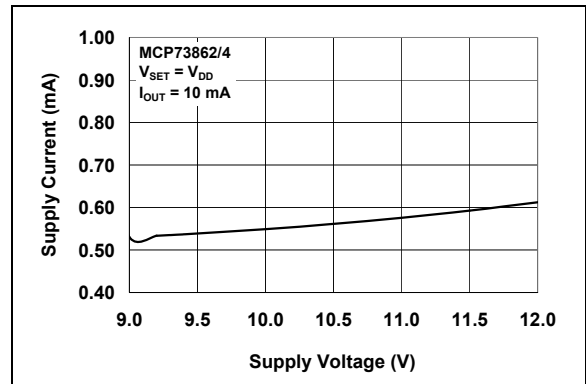
FIGURE 2-18: Supply Current ( I_{SS} ) vs. Supply Voltage ( V_{DD} ).
