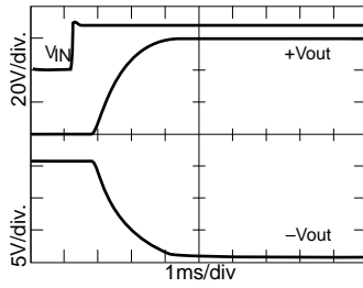
MFL2815D Turn On Response
