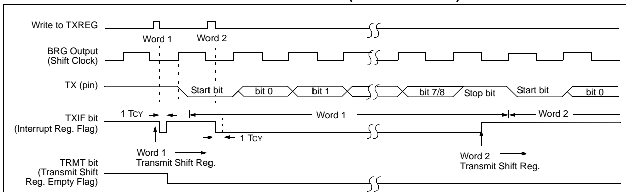
FIGURE 16-5: ASYNCHRONOUS TRANSMISSION (BACK TO BACK)
