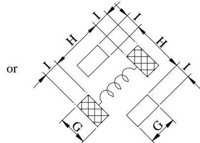
( PCB Pattern )
