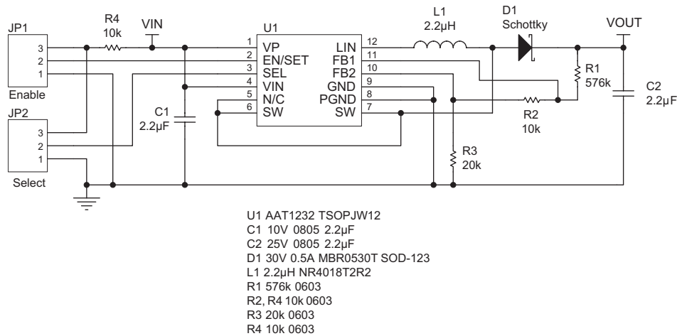
Figure 1: AAT1232 Demo Board Schematic.
