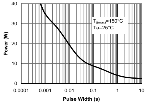
Figure 10: Single Pulse Power Rating Junction-to-Case (Note E)
