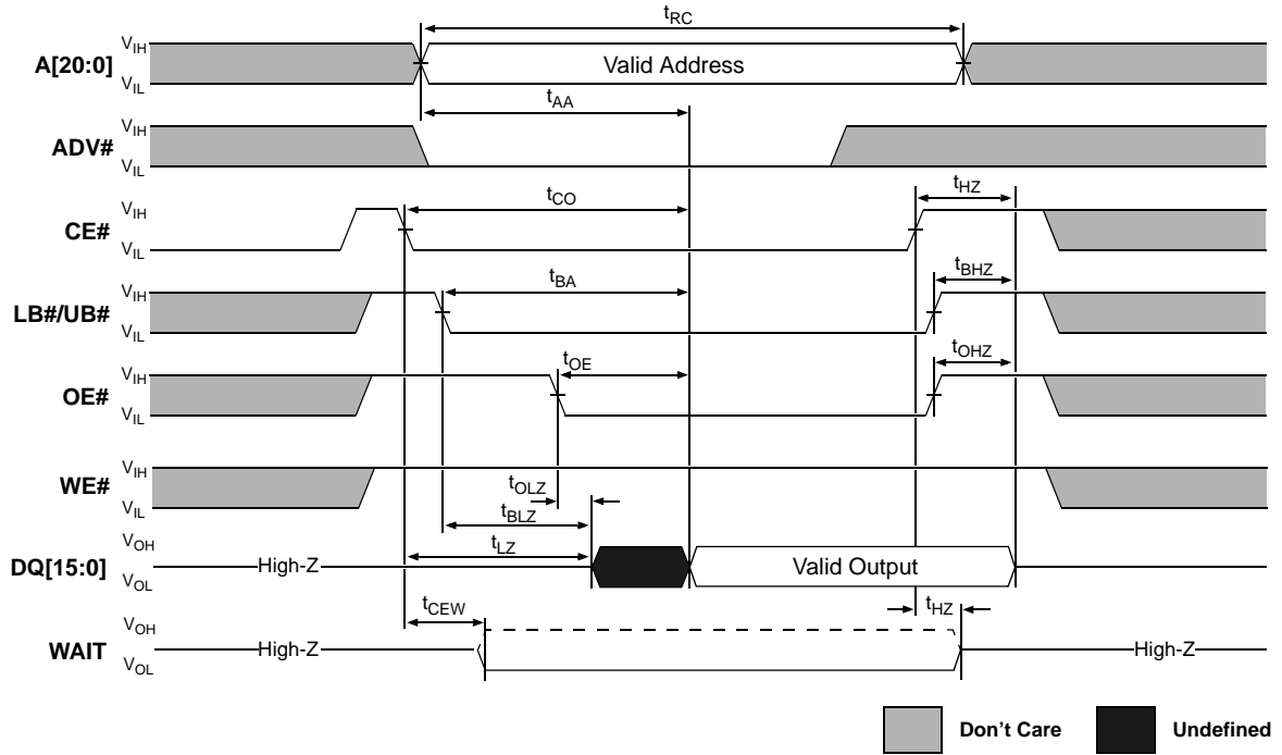
Figure 25: Asynchronous READ
