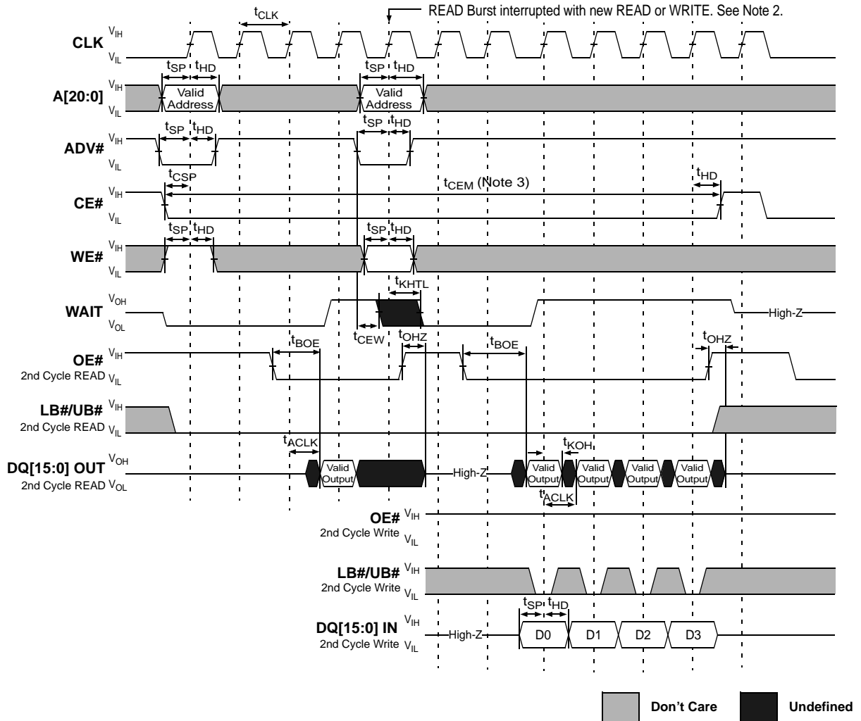
Figure 44. Burst READ Interrupted by Burst READ or WRITE
