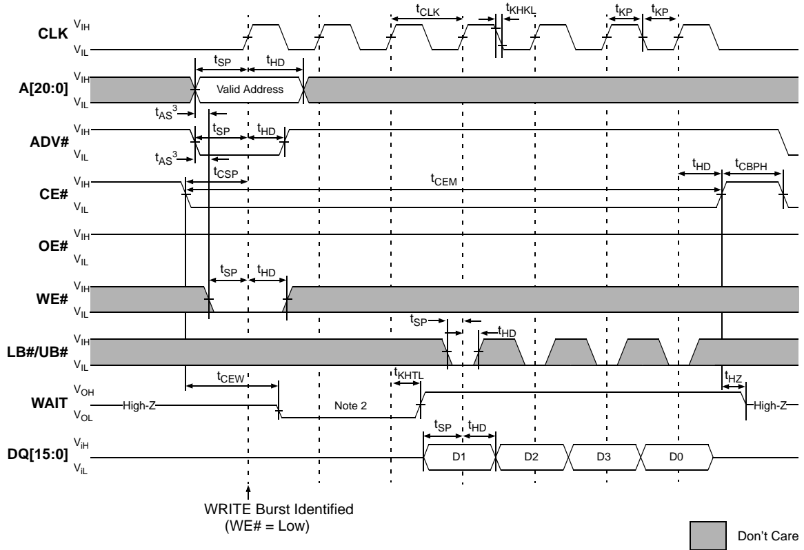
Figure 39. Burst WRITE Operation - Variable Latency Mode
