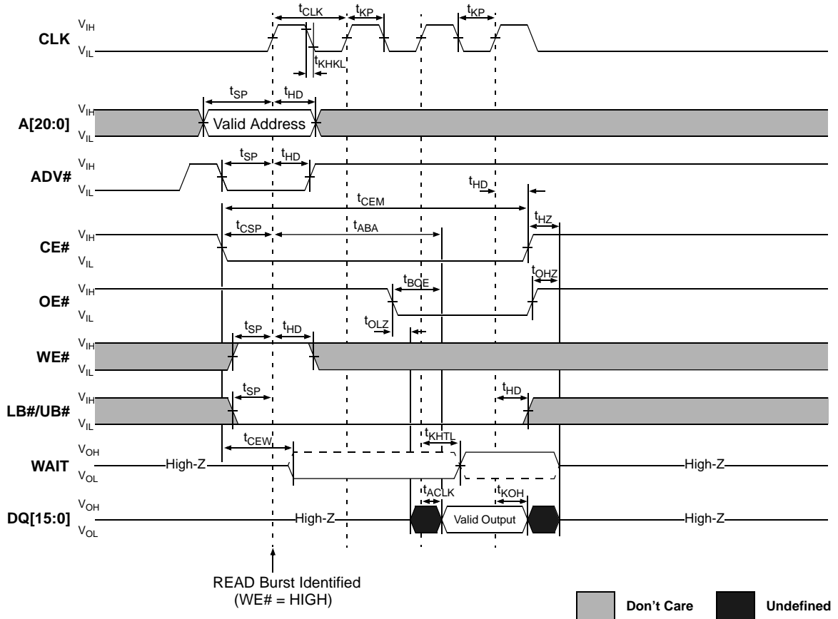
Figure 28: Single-Access Burst READ Operation - Variable Latency
