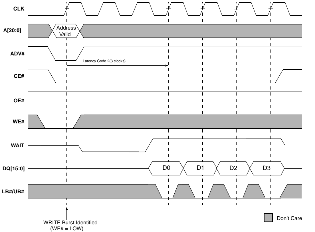
Figure 7: Burst Mode WRITE (4-word burst)
