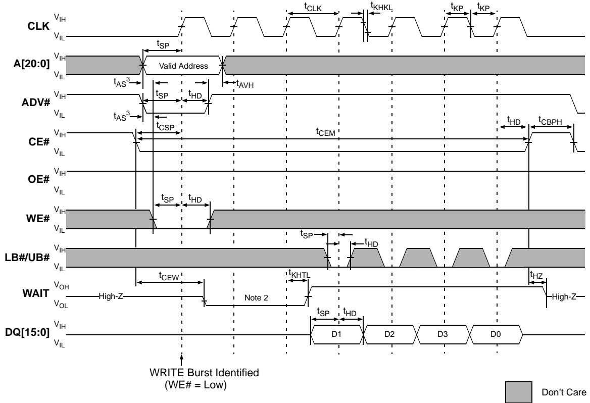
Figure 40. Burst WRITE Operation - Fixed Latency Mode
