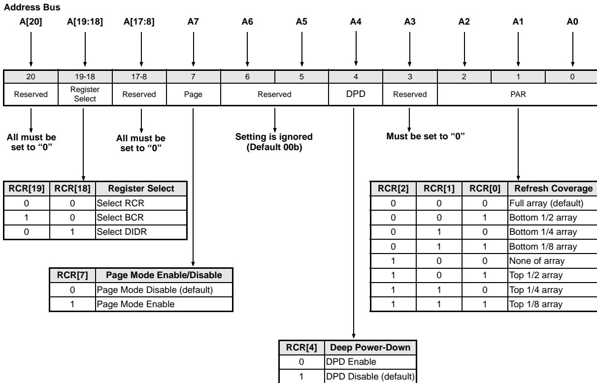
Figure 20: Refresh Configuration Register Mapping
