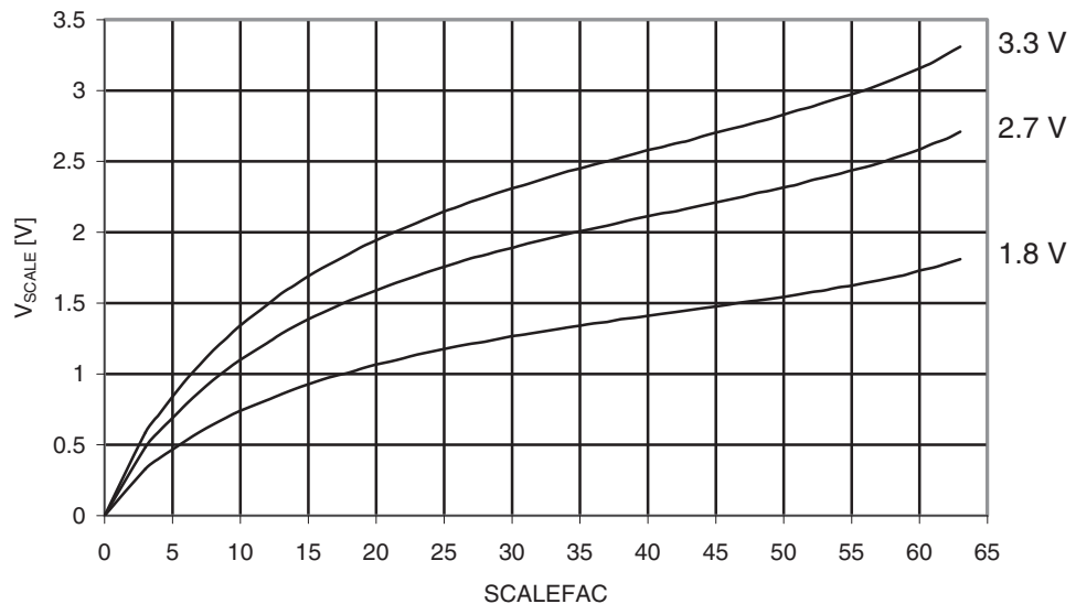
Figure 36-1. Analog Comparator Voltage Scaler vs. Scalefac T = 25°C
