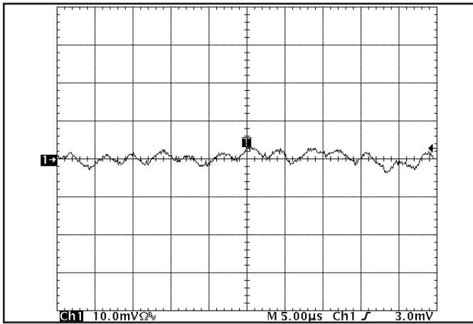
Figure 19: Input Reflected Ripple Current, i_s , through a 10\ \mu H source inductor at nominal input voltage and rated load current ( 5\ mA/div ). 1.8V and 3.3V outputs at full rated load current. (see Fig. 17)
