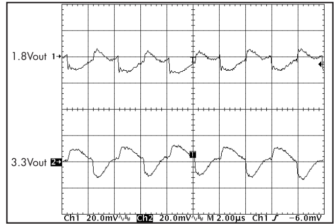
Figure 20: Output Voltage Ripple at nominal input voltage and rated load current on both outputs ( 20\ mV/div ). Load capacitance: 1\ \mu F ceramic & 15\ \mu F tantalum. Bandwidth: 20\ MHz . (see Fig. 17)
