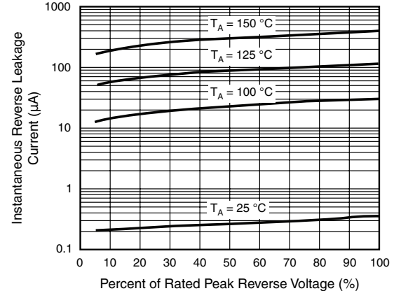
Figure 6. Typical Reverse Leakage Characteristics Per Diode
