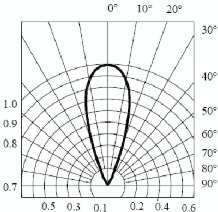
RADIATION DIAGRAM
