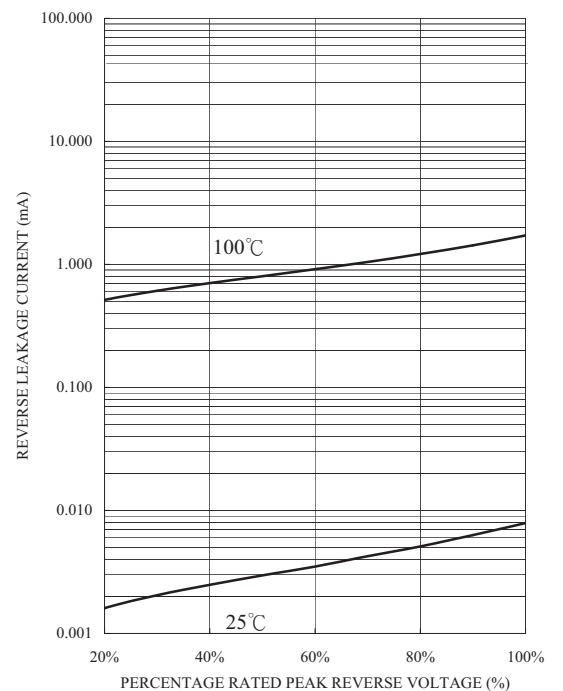
FIG. 5-TYPICAL REVERSE CHARACTERISTICS
