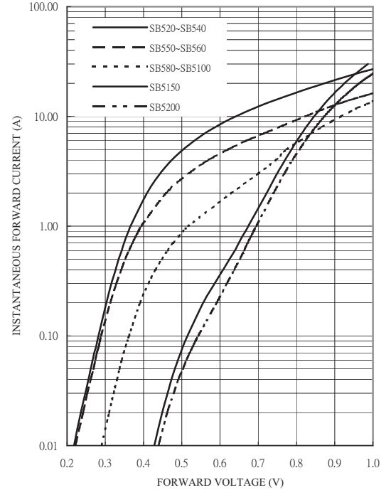
FIG. 2-TYPICAL FORWARD CHARACTERISTICS
