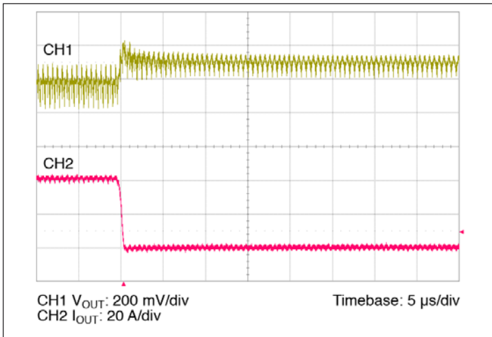
Figure 13 – 40 A – 0 A transient response; C_{IN} = 100 \mu F , no external C_{OUT}
