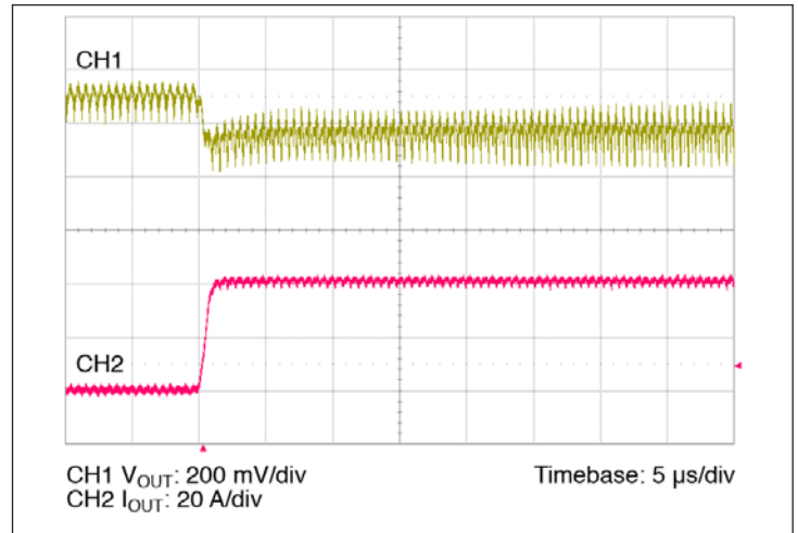
Figure 12 – 0 – 40 A transient response; C_{IN} = 100 \mu F , no external C_{OUT}
