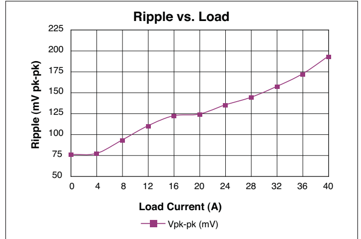
Figure 6 – V_{ripple} vs. I_{OUT} ; 45 V_{IN} ; no external output capacitance
