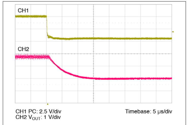
Figure 14 – PC disable waveform; R_{LOAD} = 0.045 \Omega , No external C_{OUT}
