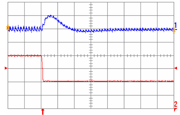
Fig. 2.5V.7: Output voltage response for V_{out} = 2.5\text{ V} to negative load current step change from 20 A to 10 A with slew rate of -5\text{ A}/\mu\text{s} at V_{in} = 12\text{ V} . Top trace: output voltage (200 mV/div.); Bottom trace: load current (5 A/div.). C_o = 100\ \mu\text{F} ceramic. Time scale: 20 \mu\text{s} /div.
