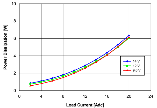
Fig. 2.5V.3: Power loss vs. load current and input voltage for V_{out} = 2.5 V converter mounted vertically with air flowing at a rate of 200 LFM (1 m/s) and T_a = 25 °C.
