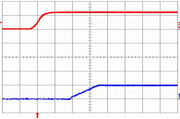
Fig. 0.7525V.4: Turn-on transient for V_{out} = 0.7525 V with application of V_{in} at full rated load current (resistive) and 100 \mu\text{F} external capacitance at V_{in} = 12 V. Top trace: V_{in} (10 V/div.); Bottom trace: output voltage (1 V/div.); Time scale: 2 ms/div.
