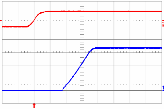
Fig. 3.3V.4: Turn-on transient for V_{out} = 3.3\text{ V} with application of V_{in} at full rated load current (resistive) and 100\text{ }\mu\text{F} external capacitance at V_{in} = 12\text{ V} . Top trace: V_{in} ( 10\text{ V/div.} ); Bottom trace: output voltage ( 1\text{ V/div.} ); Time scale: 2\text{ ms/div.}
