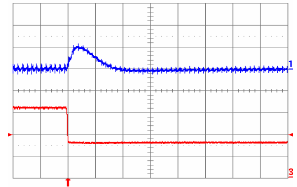
Fig. 2.0V.7: Output voltage response for V_{out} = 2.0\text{ V} to negative load current step change from 20\text{ A} to 10\text{ A} with slew rate of -5\text{ A}/\mu\text{s} at V_{in} = 12\text{ V} . Top trace: output voltage ( 200\text{ mV/div.} ); Bottom trace: load current ( 5\text{ A/div.} ). C_o = 100\ \mu\text{F} ceramic. Time scale: 20\ \mu\text{s/div.}
