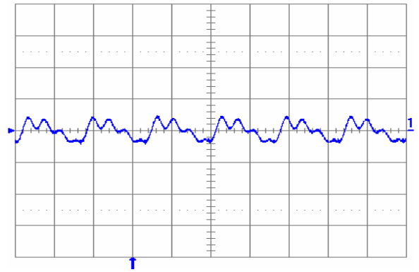
Fig. 2.0V.5: Output voltage ripple ( 20\text{ mV/div.} ) at full rated load current into a resistive load with external capacitance 100\ \mu\text{F} ceramic + 1\ \mu\text{F} ceramic and V_{in} = 12\text{ V} for V_{out} = 2.0\text{ V} . Time scale: 2\ \mu\text{s/div.}
