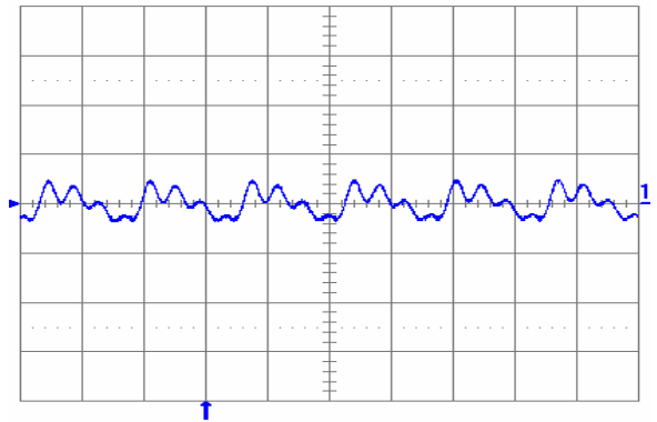
Fig. 1.8V.5: Output voltage ripple (20 mV/div.) at full rated load current into a resistive load with external capacitance 100\ \mu\text{F} ceramic + 1\ \mu\text{F} ceramic and V_{in} = 12\text{ V} for V_{out} = 1.8\text{ V} . Time scale: 2 \mu\text{s} /div.
