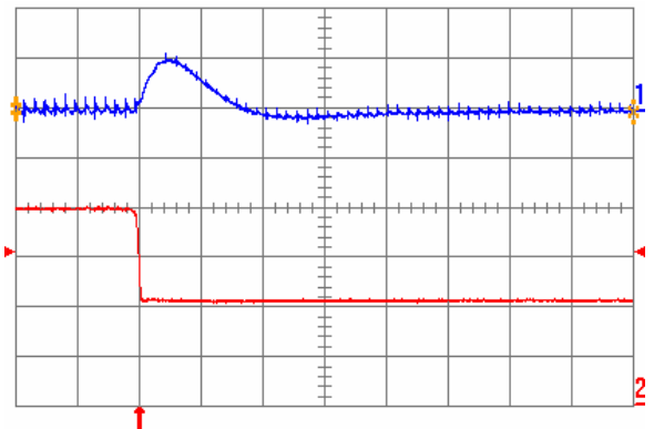
Fig. 1.0V.7: Output voltage response for V_{out} = 1.0 V to negative load current step change from 20 A to 10 A with slew rate of -5\text{A}/\mu\text{s} at V_{in} = 12 V. Top trace: output voltage (200 mV/div.); Bottom trace: load current (5 A/div.). C_o = 100 \mu\text{F} ceramic. Time scale: 20 \mu\text{s} /div.
