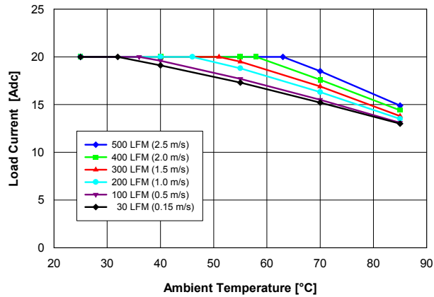
Fig. 2.5V.1: Available load current vs. ambient temperature and airflow rates for V_{out} = 2.5 V converter mounted vertically with V_{in} = 12 V, and maximum MOSFET temperature \leq 120 °C.
