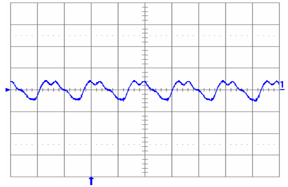
Fig. 2.5V.5: Output voltage ripple (20 mV/div.) at full rated load current into a resistive load with external capacitance 100\ \mu\text{F} ceramic + 1\ \mu\text{F} ceramic and V_{in} = 12\text{ V} for V_{out} = 2.5\text{ V} . Time scale: 2 \mu\text{s} /div.
