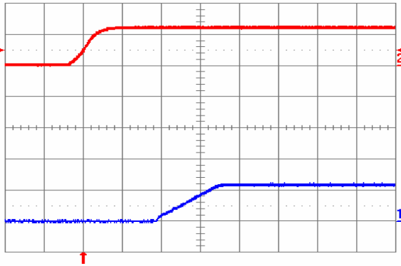
Fig. 1.2V.4: Turn-on transient for V_{out} = 1.2 V with application of V_{in} at full rated load current (resistive) and 100 \mu\text{F} external capacitance at V_{in} = 12 V. Top trace: V_{in} (10 V/div.); Bottom trace: output voltage (1 V/div.); Time scale: 2 ms/div.
