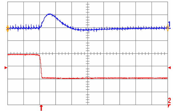
Fig. 0.7525V.7: Output voltage response for V_{out} = 0.7525 V to negative load current step change from 20 A to 10 A with slew rate of -5 \text{ A}/\mu\text{s} at V_{in} = 12 V. Top trace: output voltage (200 mV/div.); Bottom trace: load current (5 A/div.). C_o = 100 \mu\text{F} ceramic. Time scale: 20 \mu\text{s}/\text{div} .
