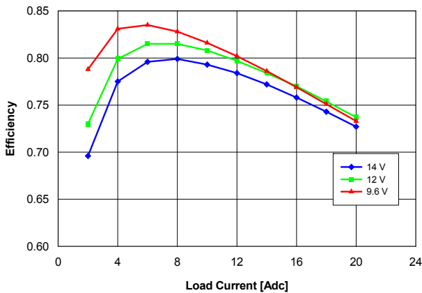
Fig. 0.7525V.2: Efficiency vs. load current and input voltage for V_{out} = 0.7525\text{ V} converter mounted vertically with air flowing at a rate of 200 LFM (1 m/s) and T_a = 25\text{ }^{\circ}\text{C} .
