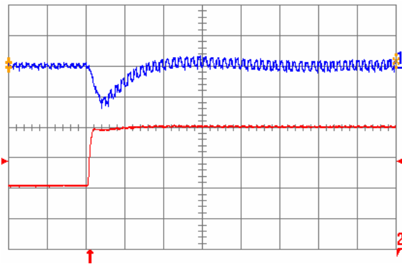
Fig. 5.0V.6: Output voltage response for V_{out} = 5.0 V to positive load current step change from 10 A to 20 A with slew rate of 5 \text{ A}/\mu\text{s} at V_{in} = 12 V. Top trace: output voltage (200 mV/div.); Bottom trace: load current (5 A/div.). C_o = 100 \mu\text{F} ceramic. Time scale: 20 \mu\text{s} /div.
