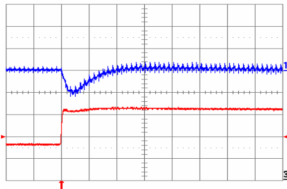
Fig. 2.0V.6: Output voltage response for V_{out} = 2.0\text{ V} to positive load current step change from 10\text{ A} to 20\text{ A} with slew rate of 5\text{ A}/\mu\text{s} at V_{in} = 12\text{ V} . Top trace: output voltage ( 200\text{ mV/div.} ); Bottom trace: load current ( 5\text{ A/div.} ). C_o = 100\ \mu\text{F} ceramic. Time scale: 20\ \mu\text{s/div.}
