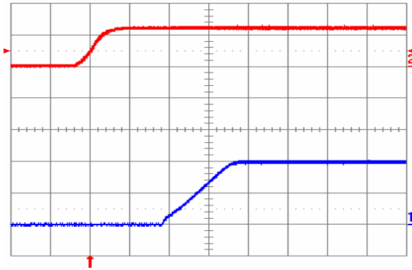
Fig. 2.0V.4: Turn-on transient for V_{out} = 2.0\text{ V} with application of V_{in} at full rated load current (resistive) and 100\ \mu\text{F} external capacitance at V_{in} = 12\text{ V} . Top trace: V_{in} ( 10\text{ V/div.} ); Bottom trace: output voltage ( 1\text{ V/div.} ); Time scale: 2\text{ ms/div.}
