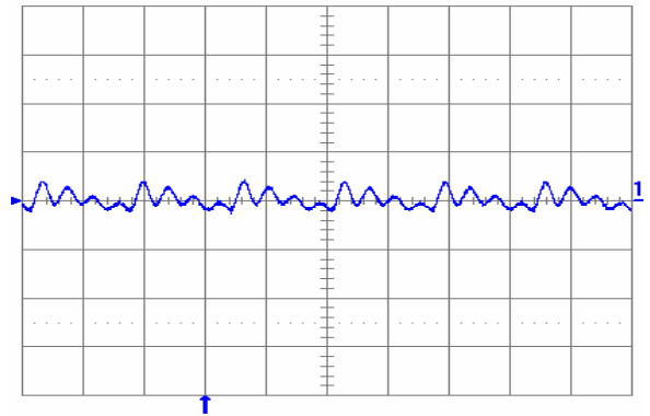
Fig. 0.7525V.5: Output voltage ripple (20 mV/div.) at full rated load current into a resistive load with external capacitance 100 \mu\text{F} ceramic + 1 \mu\text{F} ceramic and V_{in} = 12 V for V_{out} = 0.7525 V. Time scale: 2 \mu\text{s}/\text{div} .
