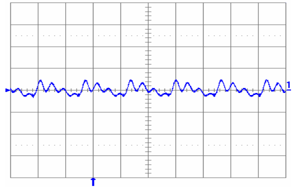
Fig. 1.5V.5: Output voltage ripple (20 mV/div.) at full rated load current into a resistive load with external capacitance 100\ \mu\text{F} ceramic + 1\ \mu\text{F} ceramic and V_{in} = 12\text{ V} for V_{out} = 1.5\text{ V} . Time scale: 2 \mu\text{s} /div.
