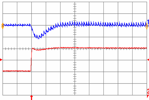
Fig. 1.8V.6: Output voltage response for V_{out} = 1.8\text{ V} to positive load current step change from 10 A to 20 A with slew rate of 5\text{ A}/\mu\text{s} at V_{in} = 12\text{ V} . Top trace: output voltage (200 mV/div.); Bottom trace: load current (5 A/div.). C_o = 100\ \mu\text{F} ceramic. Time scale: 20 \mu\text{s} /div.
