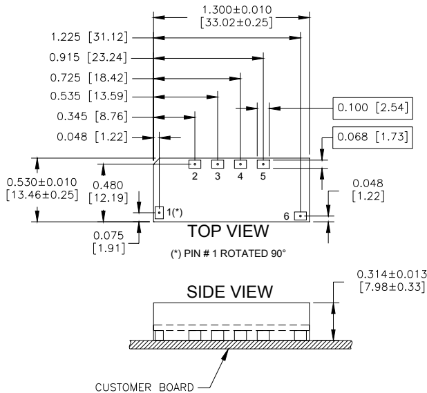
YNC12S Pinout (Surface Mount)
