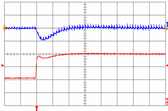
Fig. 1.0V.6: Output voltage response for V_{out} = 1.0 V to positive load current step change from 10 A to 20 A with slew rate of 5\text{A}/\mu\text{s} at V_{in} = 12 V. Top trace: output voltage (200 mV/div.); Bottom trace: load current (5 A/div.). C_o = 100 \mu\text{F} ceramic. Time scale: 20 \mu\text{s} /div.
