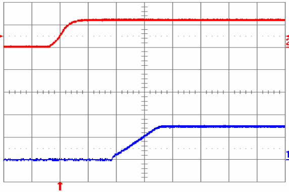
Fig. 1.5V.4: Turn-on transient for V_{out} = 1.5\text{ V} with application of V_{in} at full rated load current (resistive) and 100\ \mu\text{F} external capacitance at V_{in} = 12\text{ V} . Top trace: V_{in} (10 V/div.); Bottom trace: output voltage (1 V/div.); Time scale: 2 ms/div.
