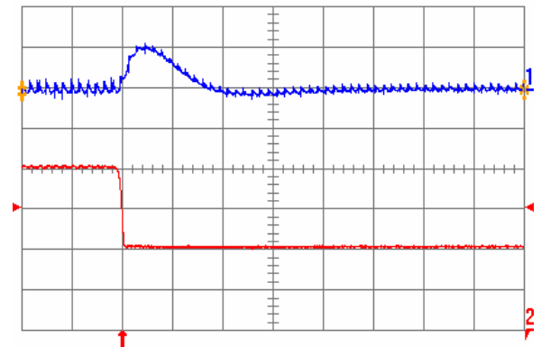
Fig. 1.8V.7: Output voltage response for V_{out} = 1.8\text{ V} to negative load current step change from 20 A to 10 A with slew rate of -5\text{ A}/\mu\text{s} at V_{in} = 12\text{ V} . Top trace: output voltage (200 mV/div.); Bottom trace: load current (5 A/div.). C_o = 100\ \mu\text{F} ceramic. Time scale: 20 \mu\text{s} /div.
