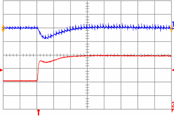
Fig. 0.7525V.6: Output voltage response for V_{out} = 0.7525 V to positive load current step change from 10 A to 20 A with slew rate of 5 \text{ A}/\mu\text{s} at V_{in} = 12 V. Top trace: output voltage (200 mV/div.); Bottom trace: load current (5 A/div.). C_o = 100 \mu\text{F} ceramic. Time scale: 20 \mu\text{s}/\text{div} .
