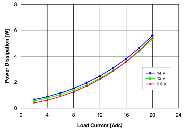
Fig. 0.7525V.3: Power loss vs. load current and input voltage for V_{out} = 0.7525\text{ V} converter mounted vertically with air flowing at a rate of 200 LFM (1 m/s) and T_a = 25\text{ }^{\circ}\text{C} .
