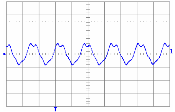
Fig. 5.0V.5: Output voltage ripple (20 mV/div.) at full rated load current into a resistive load with external capacitance 100 \mu\text{F} ceramic + 1 \mu\text{F} ceramic and V_{in} = 12 V for V_{out} = 5.0 V. Time scale: 2 \mu\text{s} /div.
