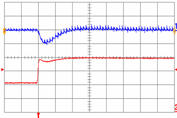
Fig. 1.2V.6: Output voltage response for V_{out} = 1.2 V to positive load current step change from 10 A to 20 A with slew rate of 5 \text{ A}/\mu\text{s} at V_{in} = 12 V. Top trace: output voltage (200 mV/div.); Bottom trace: load current (5 A/div.). C_o = 100 \mu\text{F} ceramic. Time scale: 20 \mu\text{s} /div.
