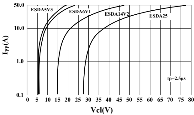
Fig.3 Clamping voltage vs peak pulse current (Tj =25°C, rectangular waveform, tp=2.5μs)
