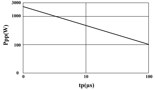
Fig.2 Peak pulse power vs exponential pulse duration(Tj =25°C)
