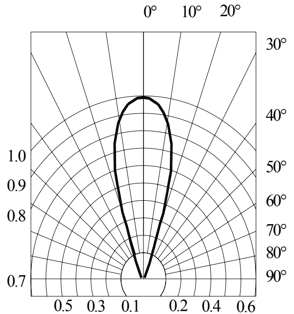
RADIATION DIAGRAM
