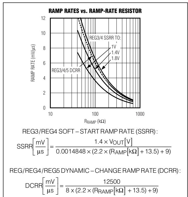
Figure 4. Soft-Start and Voltage-Change Ramp Rates
