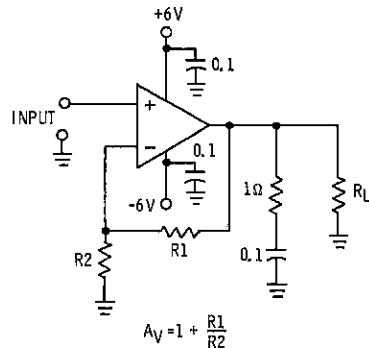
NON-INVERTING POWER AMPLIFIER
