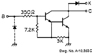
PARTIAL SCHEMATIC
