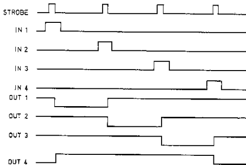
UNIPOLAR WAVE DRIVE
