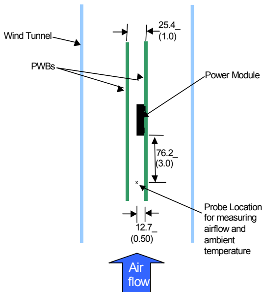
Figure 33. Thermal Test Up
