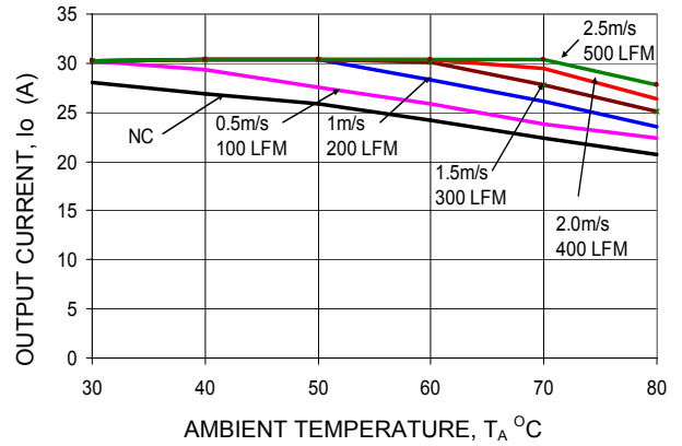
Figure 4. Derating Output Current versus Ambient Temperature and Airflow (ATM030A0X3-SR).
