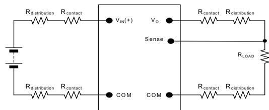
Figure 30. Effective Circuit Configuration for Remote Sense operation.
