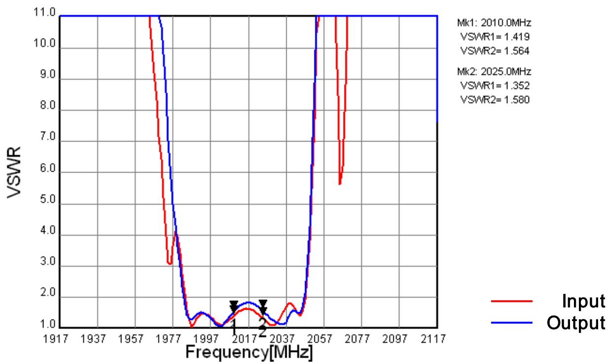
Fig.2 VSWR
