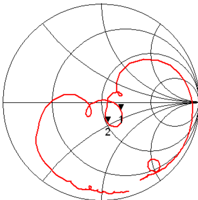
Fig.5 Impedance (S11)
