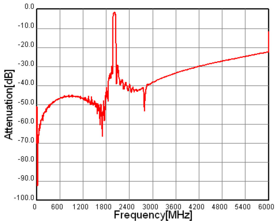
Fig.4 Wide-band Characteristic
