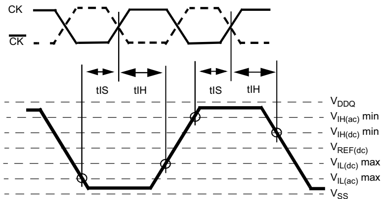
Differential input waveform timing - t_{IS} and t_{IH}
