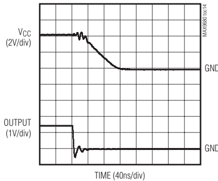
TURN-OFF TIME
