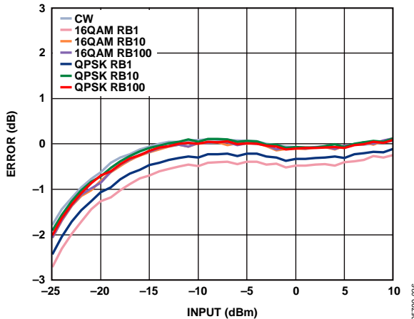
Figure 26. Error from CW Linear Reference vs. Input with Various LTE Reverse Link Waveforms at 2600 MHz, C_{OUT} = \text{Open}
