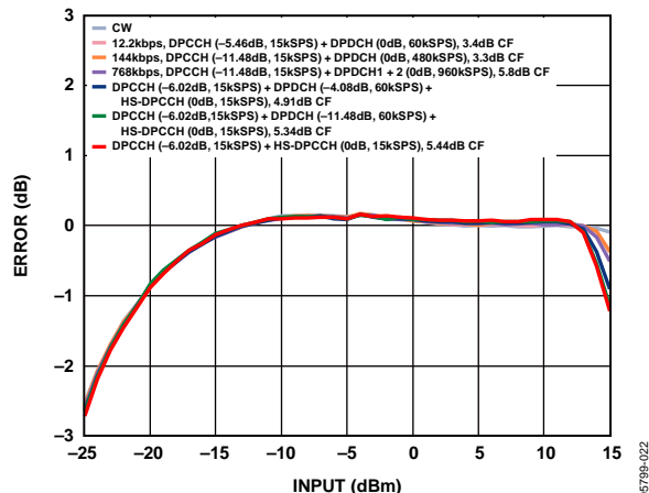
Figure 22. Error from CW Linear Reference vs. Input with Various W-CDMA Reverse Link Waveforms at 900 MHz, C_{OUT} = \text{Open}
