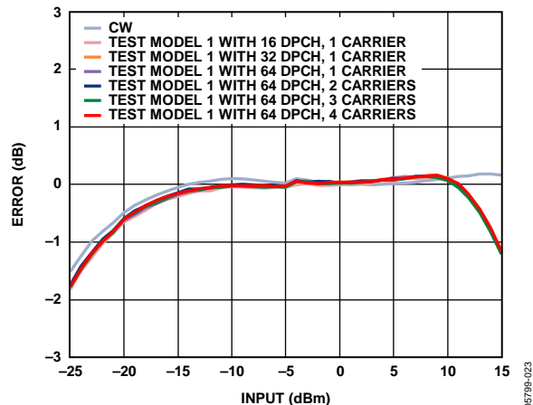
Figure 23. Error from CW Linear Reference vs. Input with Various W-CDMA Forward Link Waveforms at 2200 MHz, C_{OUT} = \text{Open}
