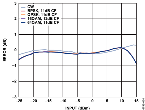
Figure 24. Error from CW Linear Reference vs. Input with Various 802.16 OFDM Waveforms at 3500 MHz, 10 MHz Signal BW, and 256 Subcarriers for All Modulated Signals, C_{OUT} = \text{Open}
