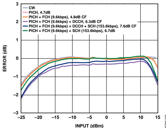
Figure 25. Error from CW Linear Reference vs. Input with Various CDMA2000 Reverse Link Waveforms at 1900 MHz, C_{OUT} = \text{Open}
