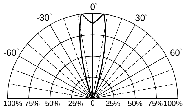
Fig.6 Directive Radiation
