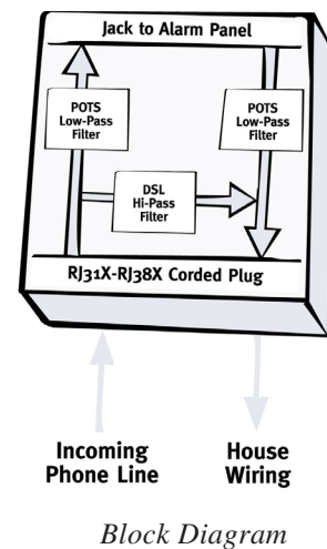
Z-BLOCKER® Z-A431PJ31X Alarm Panel DSL Filter
