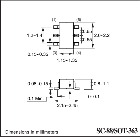
SC-88/SOT-363
