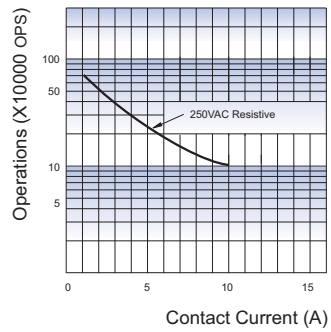
EDURANCE CURVE
