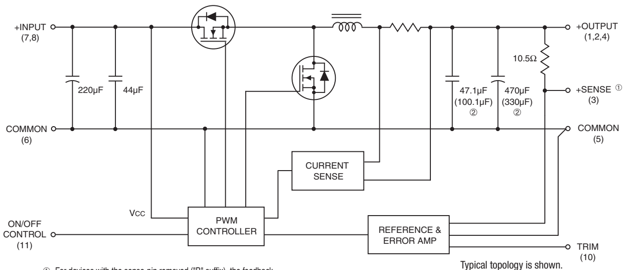
Figure 1. Simplified Schematic
