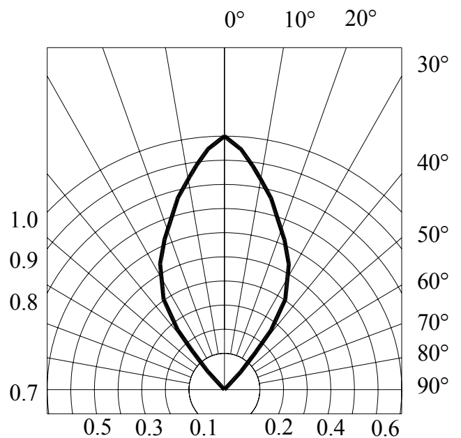
Radiation Diagram
